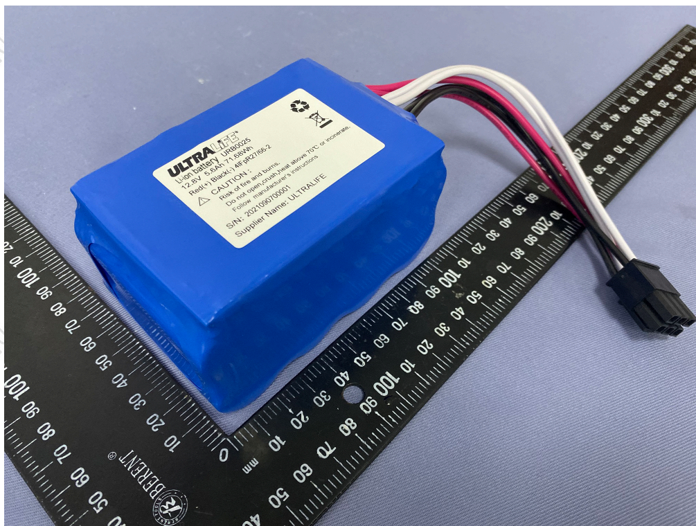
Figure 1 Overall view I of battery (电池组图I)
